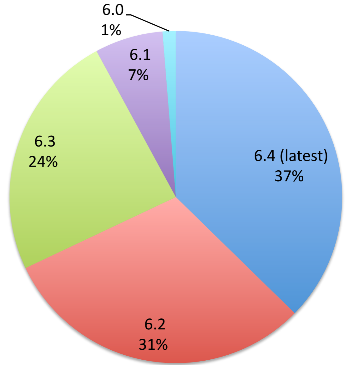
Drupal 6
