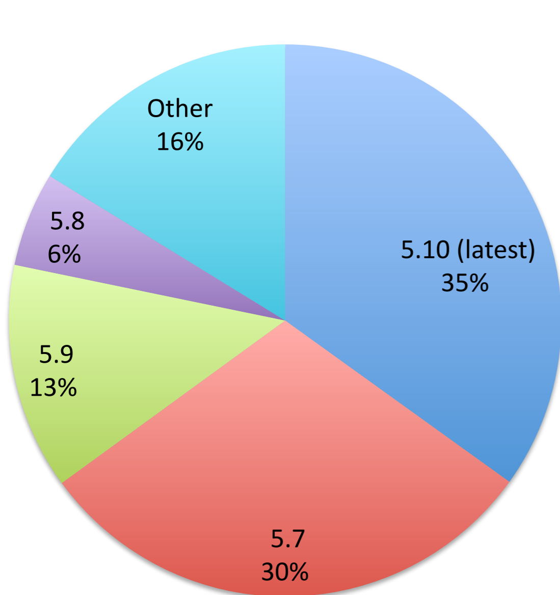
Drupal 5
